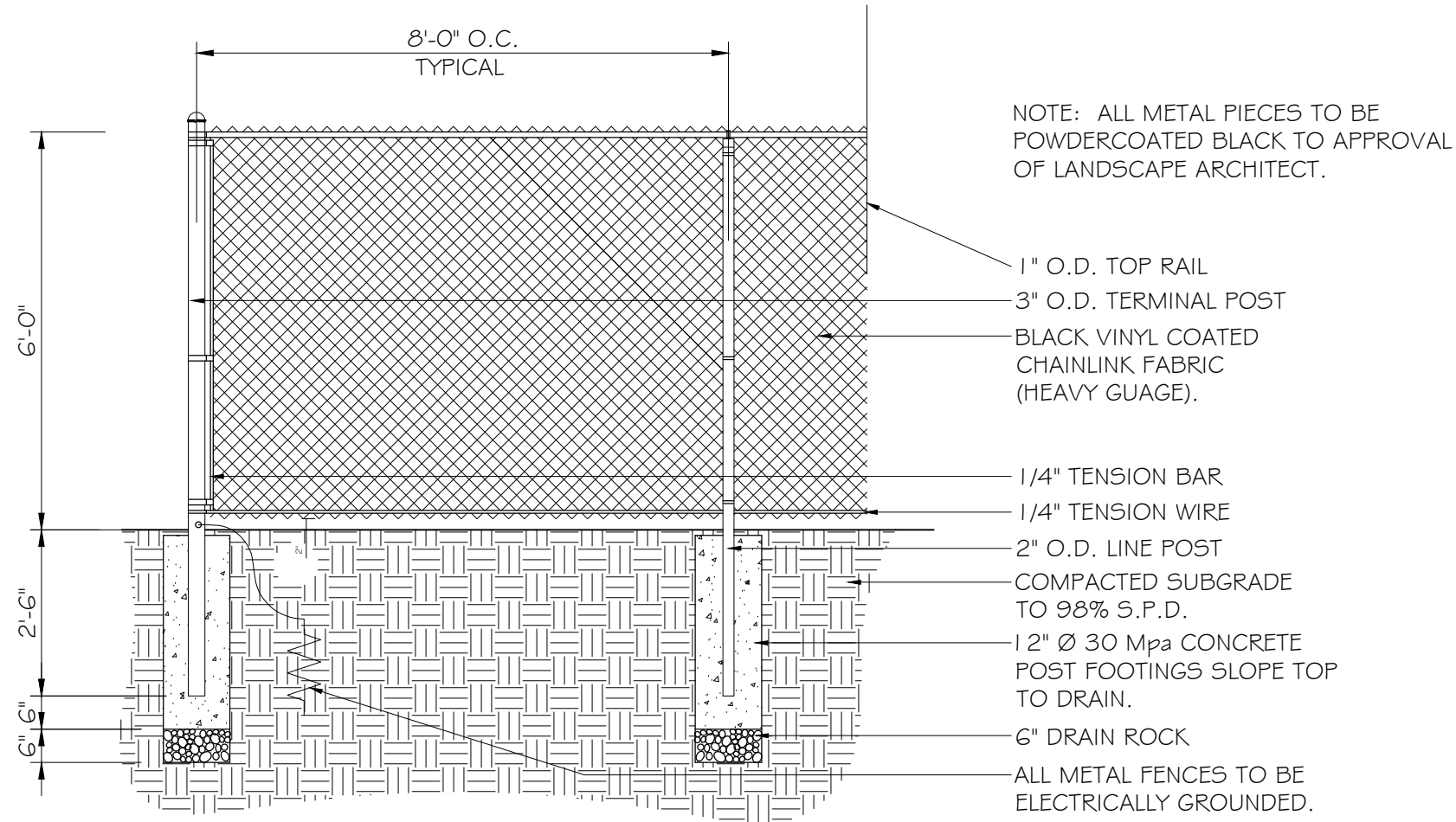
2 L2 SCALE 1:30 CHAINLINK FENCE
