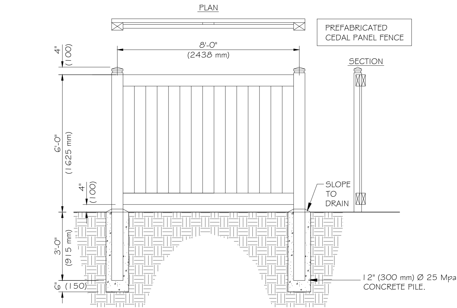
1 L2 SCALE 1:30 PREFAB CEDAR PANEL PERIMETER WOOD FENCE
